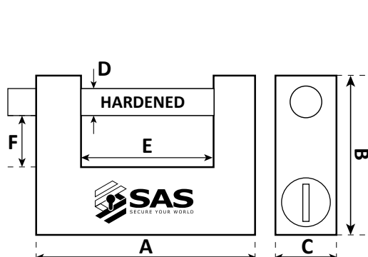
KB21 UNILOCK
